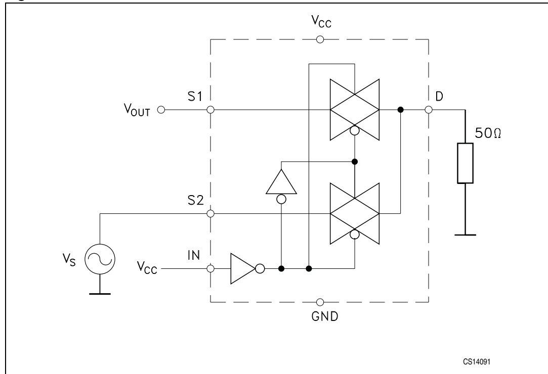
Figure 7. Channel-to-channel crosstalk
